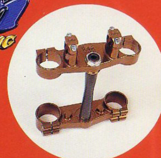
Piastra forcella ricavata dal pieno optional. Front fork triple clamp machined from block.
